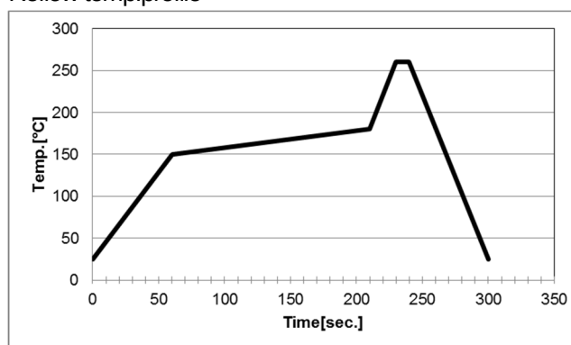
Reflow temp.profile
